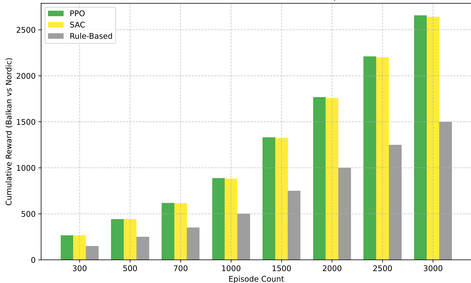
Cumulative Reward (Balkan vs Nordic) Across Episode Counts
